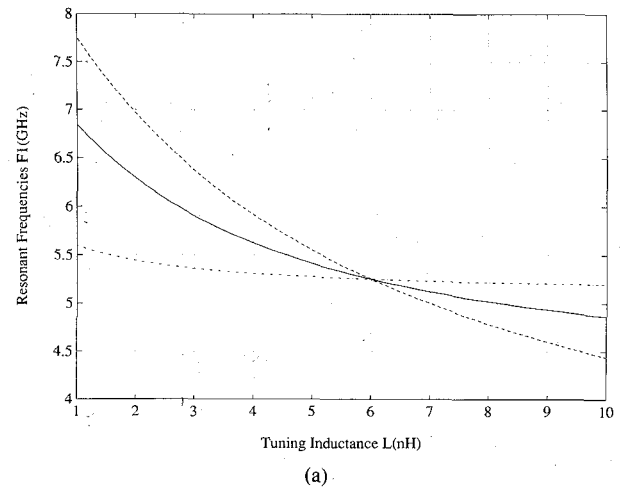
Fig. 3. Resonant frequencies of the serially and parallel tuned front ends as function of tuning inductances. Dashed line: resonant frequency of the serially tuned front end. Solid line: resonant frequency of the parallel tuned front end.
