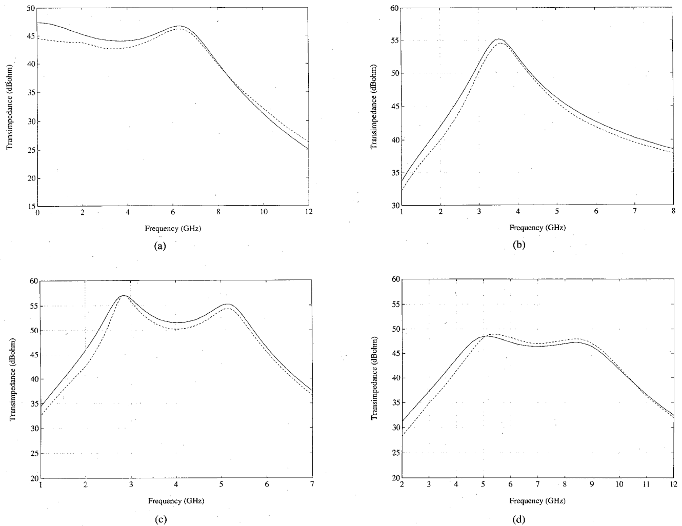
Fig. 6. (a) Comparison between the calculated and simulated transimpedances of the serially tuned front end. Solid line: calculated result. Dashed line: simulated result. L_s = 6.0 nH, R_b = 200 \Omega . (b) Comparison between the calculated and simulated transimpedances of the parallel tuned front end. Solid line: calculated result. Dashed line: simulated result. L_p = 6.0 nH. (c) Comparison between the calculated and simulated transimpedances of the transformer tuned front end. Solid line: calculated result. Dashed line: simulated result. L_p = L_{s1} = L_{s2} = 6.0 nH. (d) Comparison between the calculated and simulated transimpedances of the mixed tuned front end. Solid line: calculated result. Dashed line: simulated result. L_{p1} = L_{p2} = L_s = 6.0 nH.
